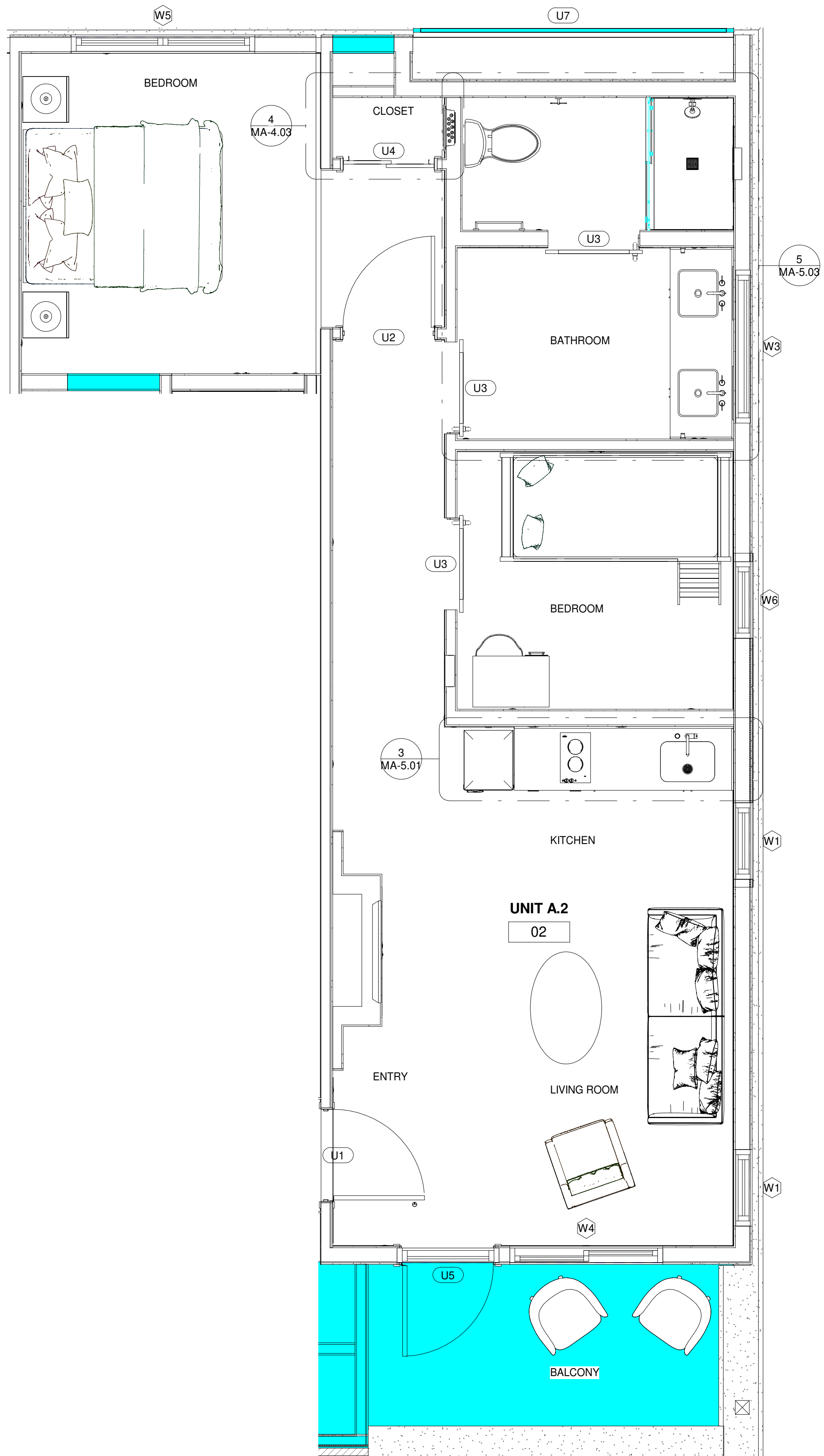
2 ENLG FF&E - UNIT A.2 3/8" = 1'-0"
